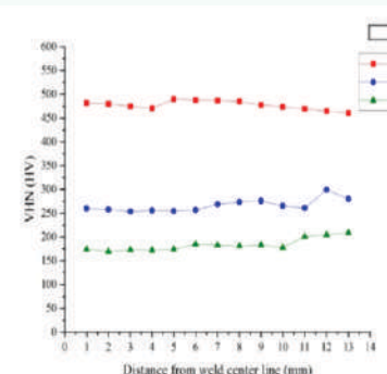
Micro-hardness welded joints across the weld center line
