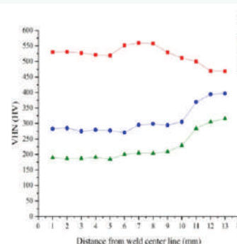
Micro-hardness welded joints across the weld center line
