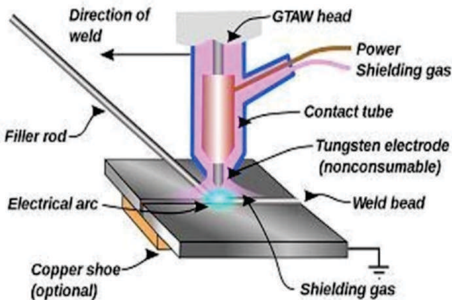
Schematics shows the GTA welding process
